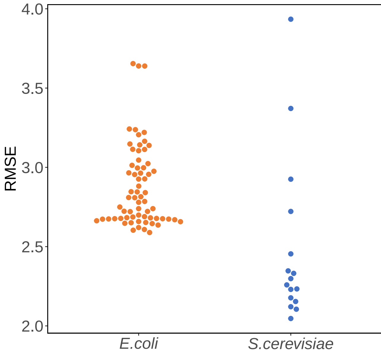
RMSE between \log_{10}K and \log_{10}CAQ (EOI) for glycolysis enzymes in E.coli and S.cerevisiae
